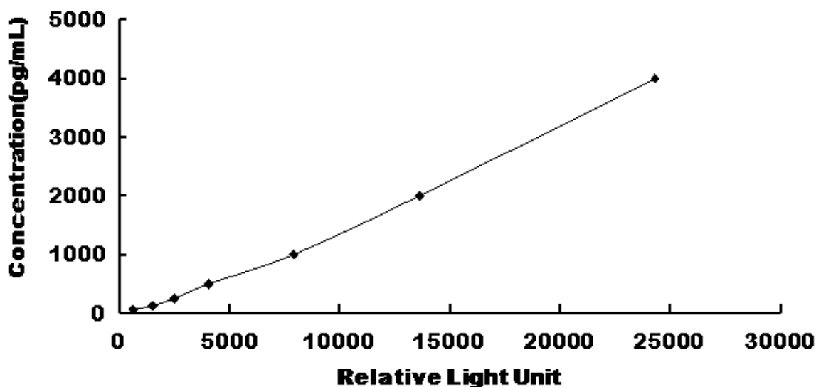
Typical Standard Curve for Rat BMP2 CLIA.
